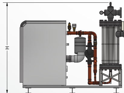
SIDE VIEW 400-500
